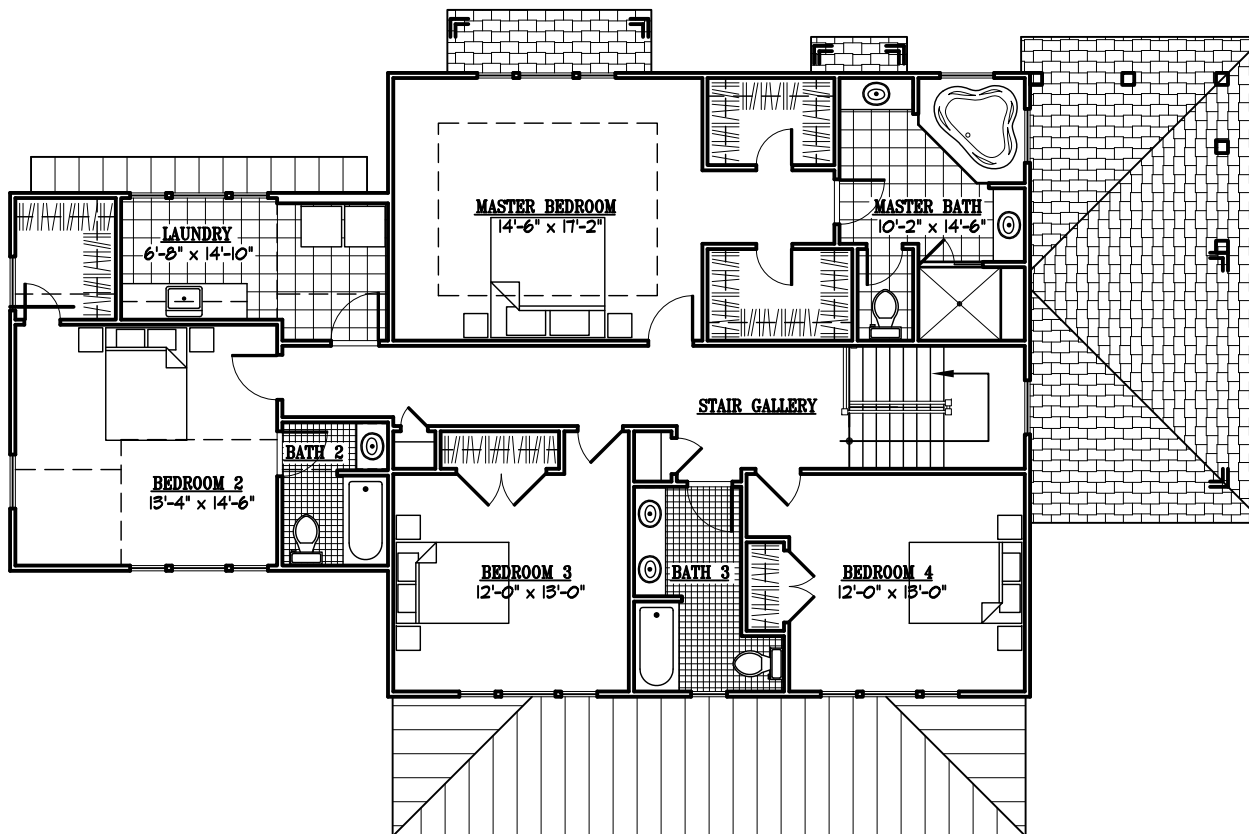
4 SECOND FLOOR PLAN 1,671 SQ. FT.
